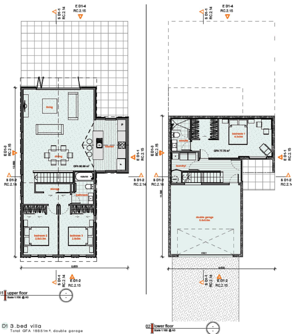
TYPE D1 TYPOLOGY FLOOR PLAN & PERSPECTIVES
